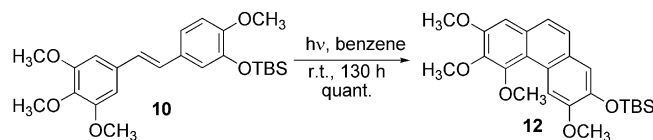
Scheme 4. Photochemical cyclization of trans -stilbene 10 .
