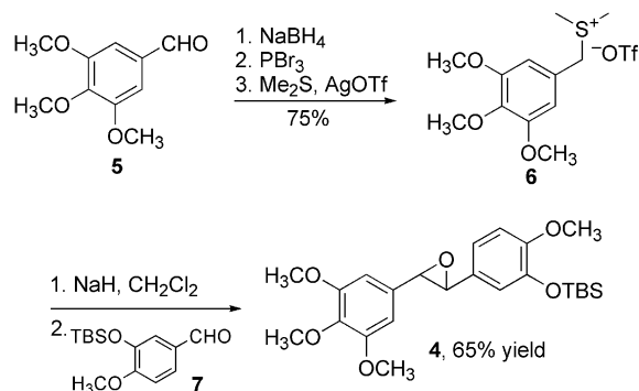
Scheme 1. Synthesis of trans -epoxide 4 .
