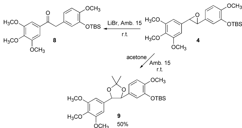
Scheme 2. Elaboration of trans -epoxide 4 .
