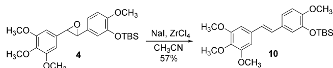
Scheme 3. Deoxygenation of trans -epoxide 4 .
